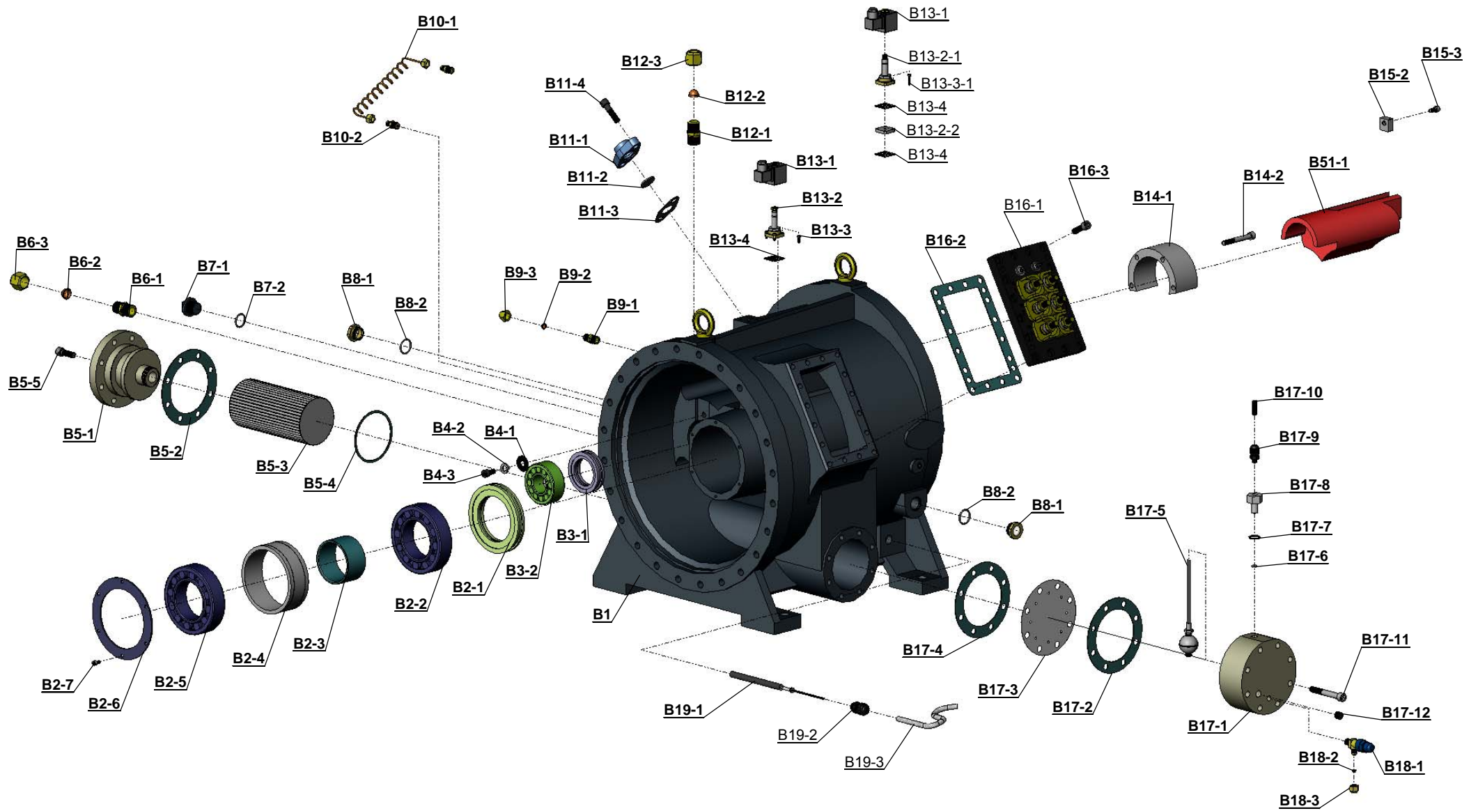
LA-610,710~930 B - Compression Casing
